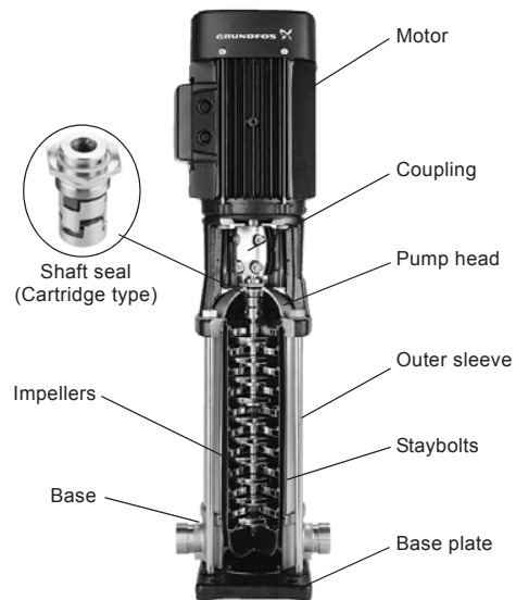
Fig. 2 CR pump
