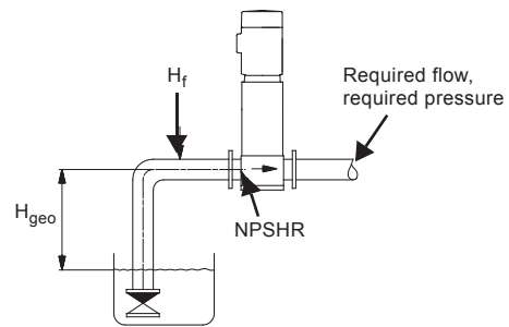
Fig. 9 Sizing data
