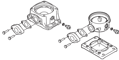
Oval flange
