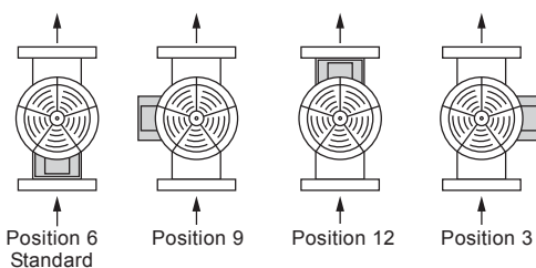
Fig. 3 Terminal box positions
