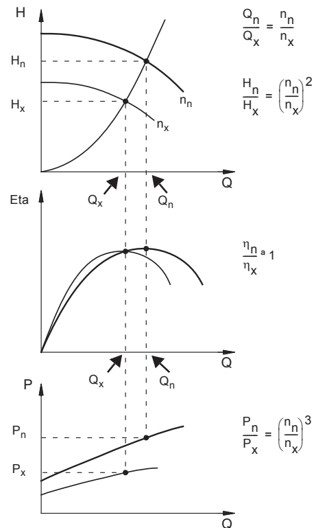
Fig. 13 Affinity equations
